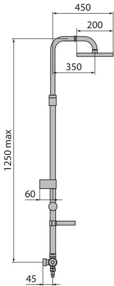
Shower head dimensions / Ducha fija 200x200 mm
